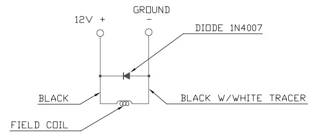
CIRCUIT DIAGRAM
